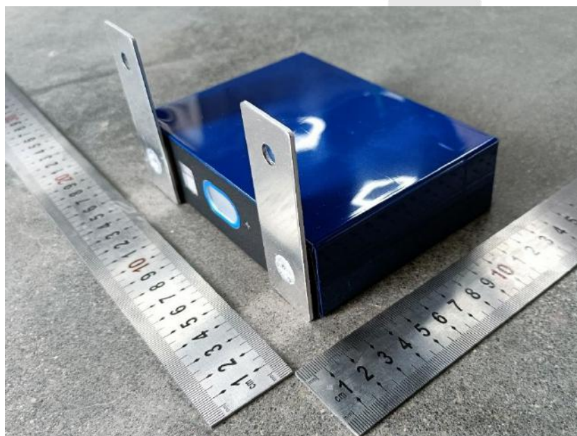
Picture 4 Front view of cell
